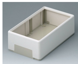
A9540165 FLAT-PACK CASE 210 A АБС (UL 94 HB) белый RAL 9002 210x125x70mm IP 40
