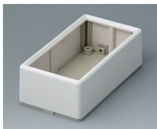
A9520165 FLAT-PACK CASE 120 A АБС (UL 94 HB) белый RAL 9002 120x65x40mm IP 40
